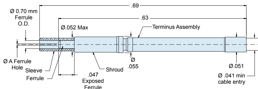
181-064 Socket Terminus
