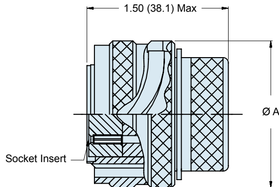
06 Plug Adapter U.S. PATENT NO. 5,960,137
