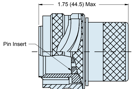
06 Plug Adapter U.S. PATENT NO. 5,960,137
