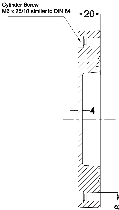
SECTION B-B
