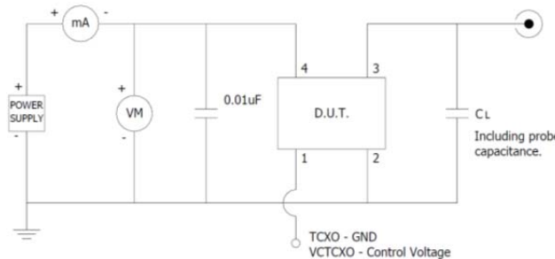
TEST CIRCUIT - HCMOS LOAD
