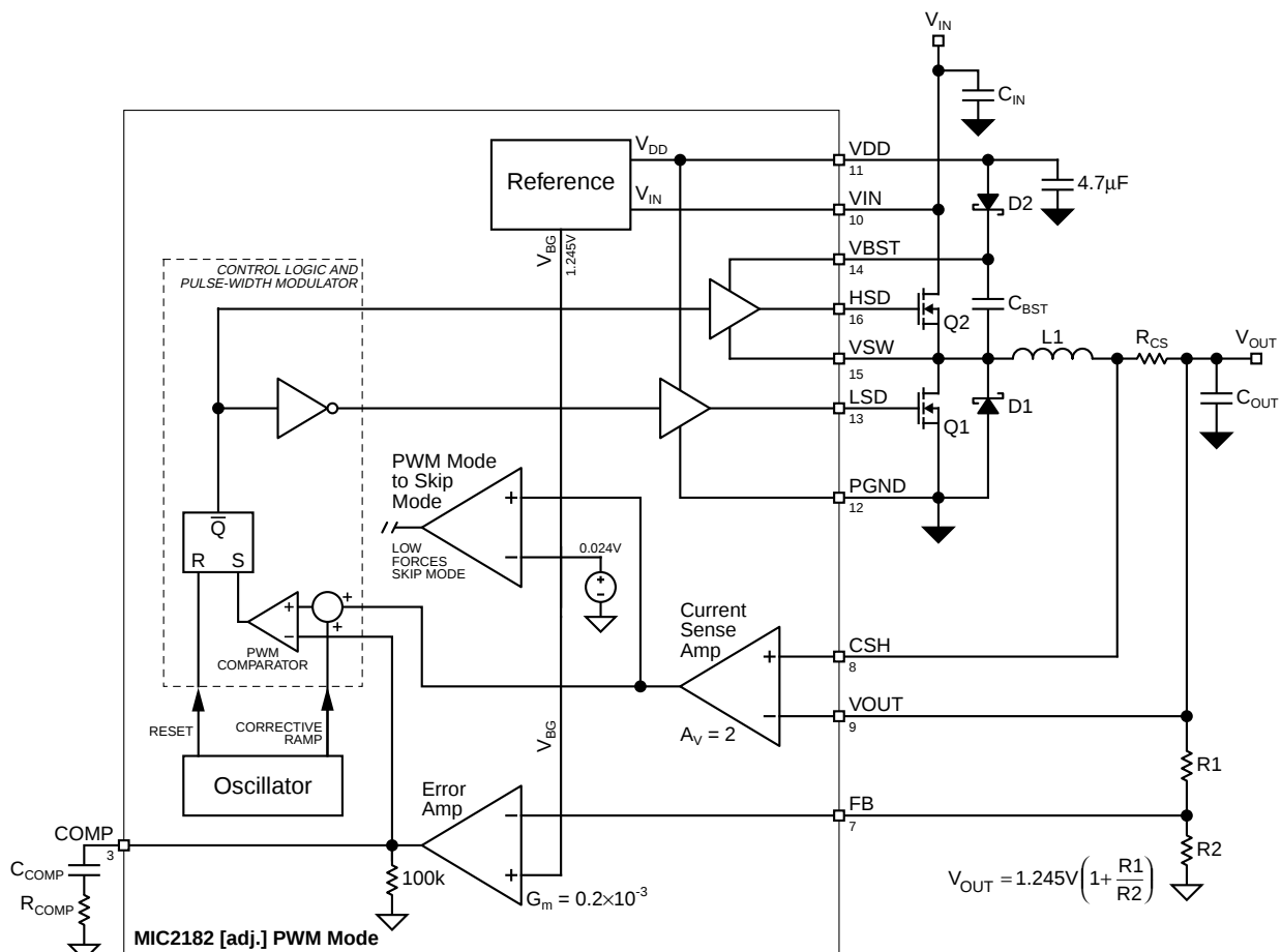
Figure 3. PWM Operation
