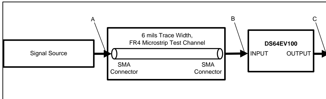
Figure 2. Test Setup Diagram
