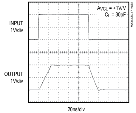
MAX4434/MAX4436 LARGE-SIGNAL PULSE RESPONSE
