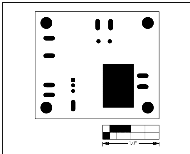
Figure 11. MAX17502F EV Kit PCB Layout—Bottom Solder Mask
