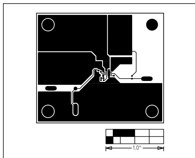
Figure 8. MAX17502F EV PCB Layout—Component Side
