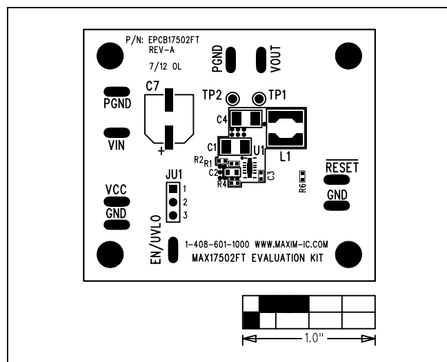
Figure 7. MAX17502F EV Kit Component Placement Guide—Component Side
