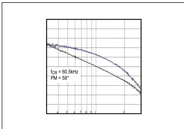
Figure 3. MAX17502F Full Load Bode Plot ( V_{IN} = 24\text{V} )
