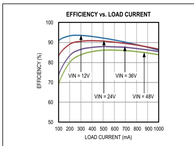
Figure 2. MAX17502F Efficiency
