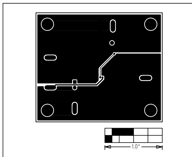
Figure 9. MAX17502F EV Kit PCB Layout—Solder Side
