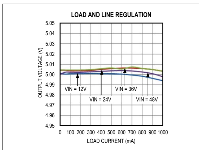
Figure 1. MAX17502F Load and Line Regulation
