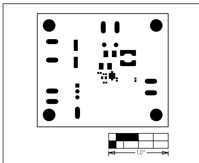
Figure 10. MAX17502F EV Kit PCB Layout—Top Solder Mask
