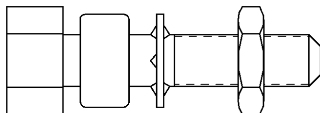
ASSEMBLED VIEW
