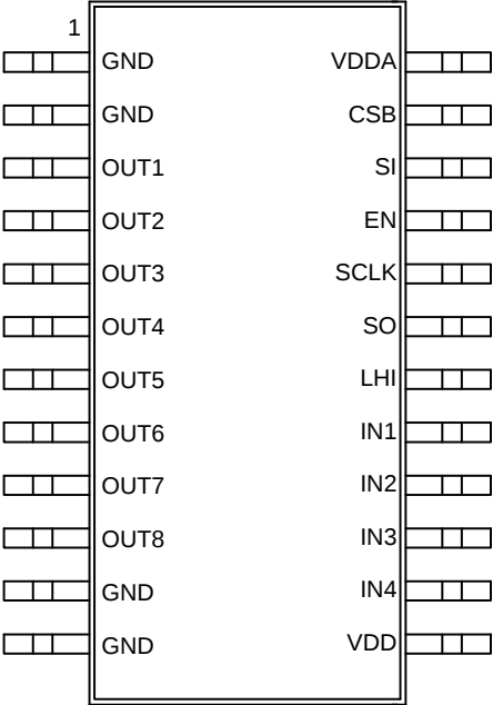
Figure 3. Pinout
