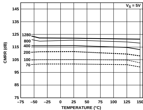
Figure 20. CMRR vs. Temperature at Different Gains
