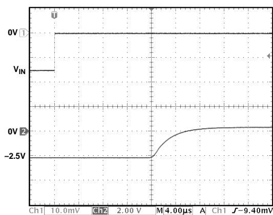
Figure 44. Negative Overload Recovery (Gain = 1280)
