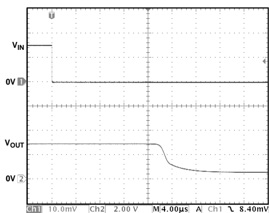
Figure 45. Positive Overload Recovery (Gain = 1280)
