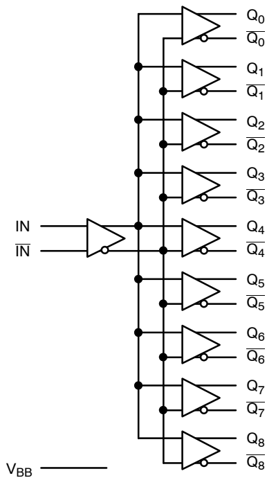
Figure 2. Logic Symbol
