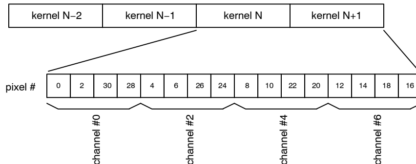
Figure 43. Data Output Order for 4 LVDS Output Channels in Subsampling Mode on a Monochrome Sensor
