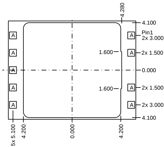
A= 0.600 x 0.600 mm BOTTOM PIN VIEW
