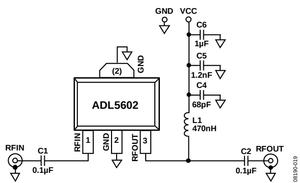
Figure 20. Evaluation Board Schematic
