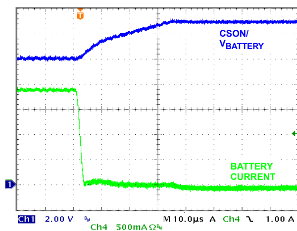
FIGURE 11. BATTERY REMOVAL
