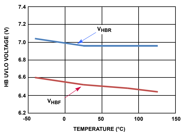
FIGURE 18. V_{\text{HB}} UNDERVOLTAGE LOCKOUT THRESHOLD vs TEMPERATURE
