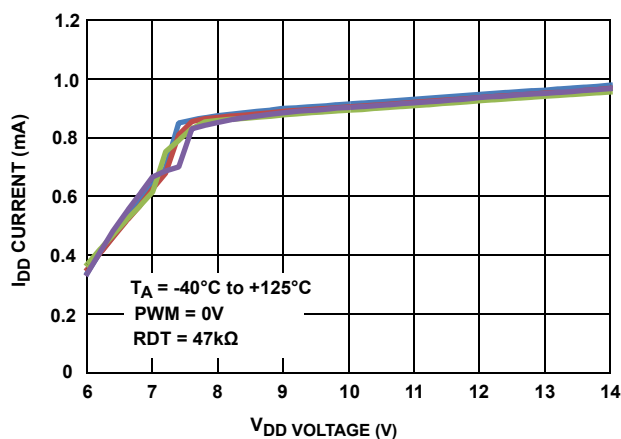
FIGURE 21. I_{\text{DD}} QUIESCENT CURRENT vs SUPPLY VOLTAGE
