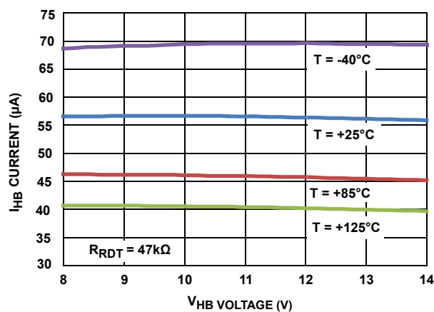
FIGURE 22. I_{\text{HB}} QUIESCENT CURRENT vs VOLTAGE
