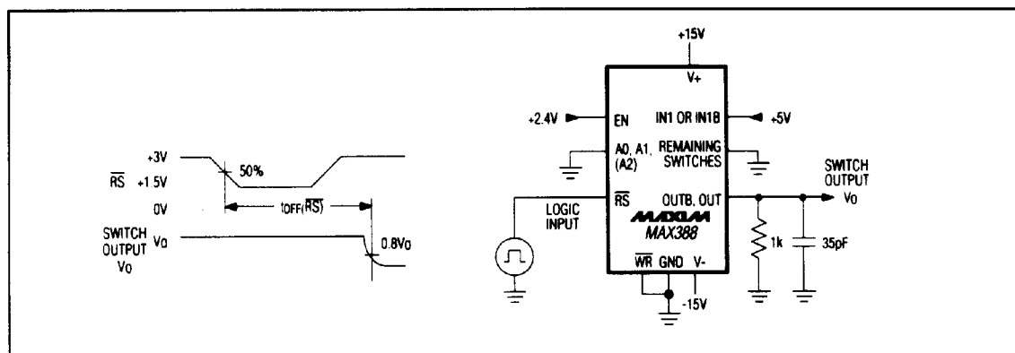
Figure 6. Reset Turn-Off Time ( t_{OFF}(RS) )
