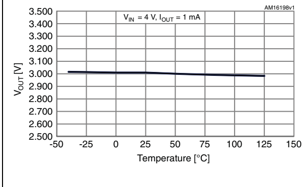
Figure 7. Output voltage vs. temp. for fixed version ( I_O = 1 \text{ mA} )
