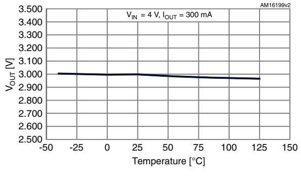
Figure 8. Output voltage vs. temp. for fixed version ( I_O = 300 \text{ mA} )
