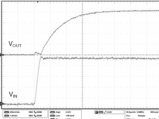
Figure 30. Startup transient
