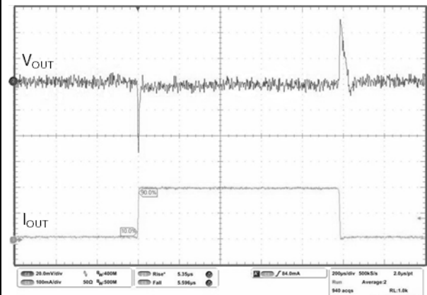
Figure 29. Load transient ( V_{OUT} = V_{ADJ} )
