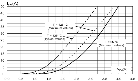
Figure 2: Forward voltage drop versus forward current
