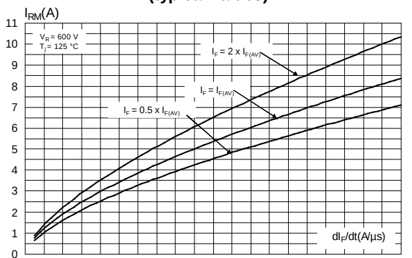
Figure 5: Reverse recovery current versus di_F/dt (typical values)
