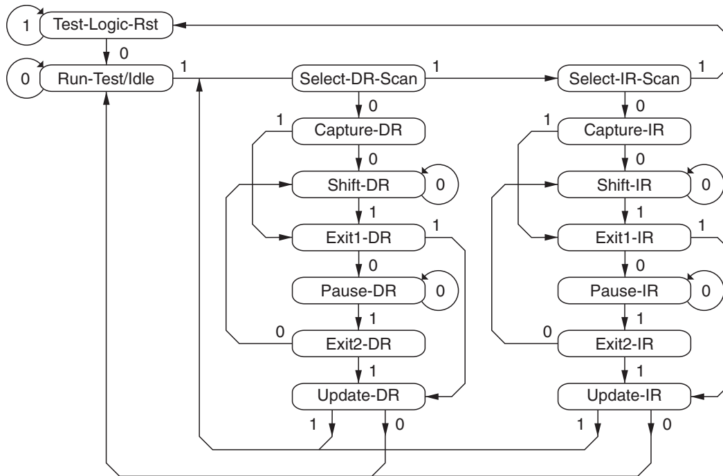
Figure 5-31. TAP States
