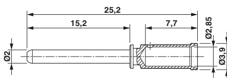
Dimensioned drawing
