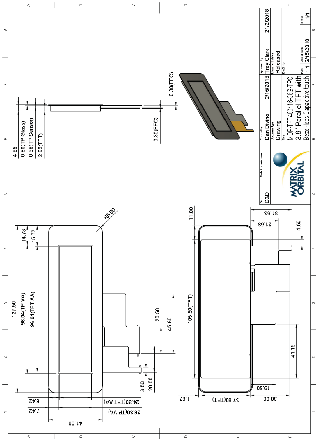
Figure 1: MOP-TFT480116-38G-BLH-TPC Drawing
