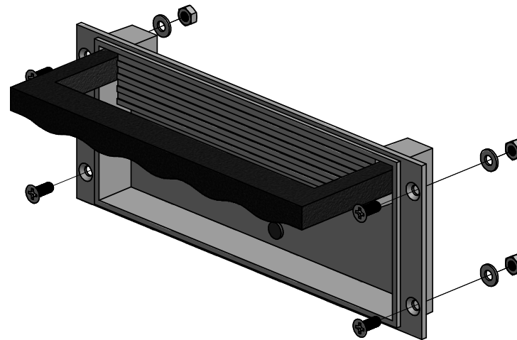
ISO VIEW WITH HANDLE OPEN
