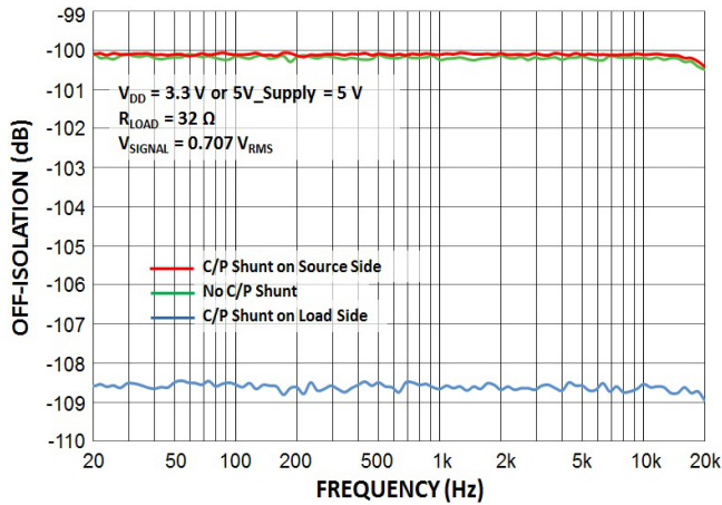
Figure 14. Off-Isolation, 0.707 V RMS Signal, 32 \Omega Load
