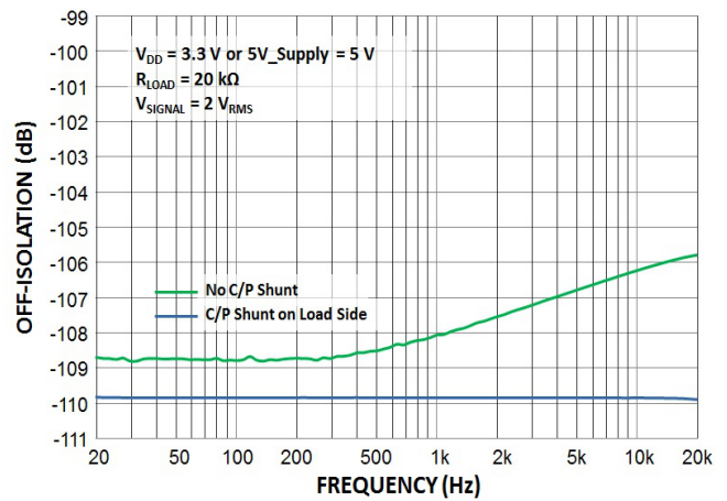
Figure 13. Off-Isolation, 2 V RMS Signal, 20 k \Omega Load
