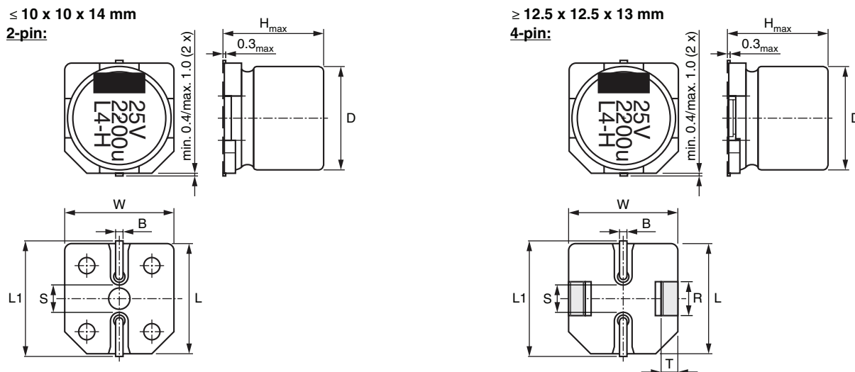
Fig.2 Dimensional outline
