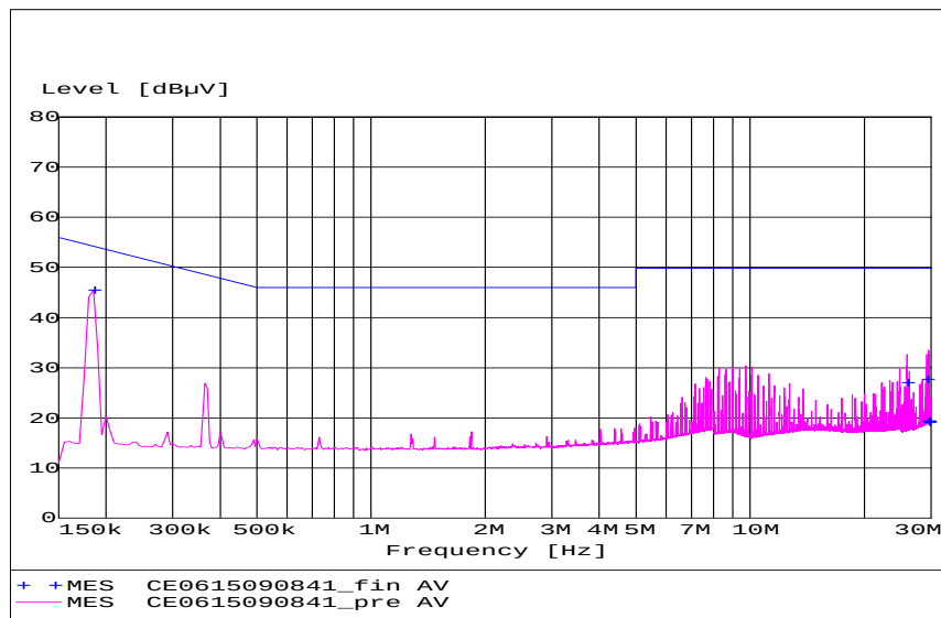
Figure 25. EMC Considerations
