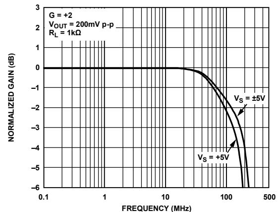
Figure 3. Frequency Response; G = \pm 2 , V_S = +5 V or -5 V
