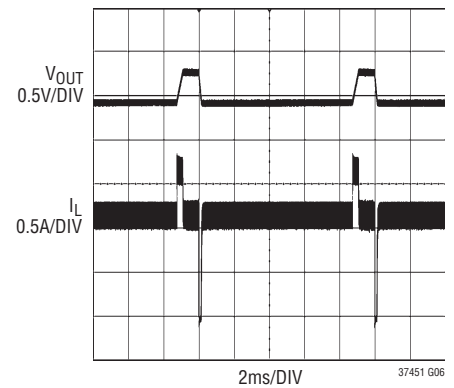
Adaptive LED Bus Voltage I
