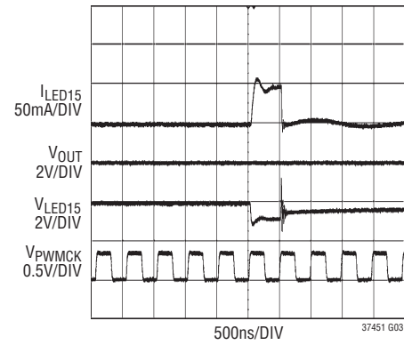
500Hz 4096:1 GS Dimming
