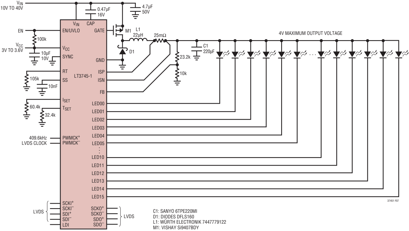
Figure 7. 16-Channel LED Driver, 500kHz Buck, 1 LED 25mA to 75mA per Channel, 100Hz 12-Bit Dimming
