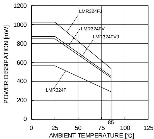
Figure 50. Derating curve
