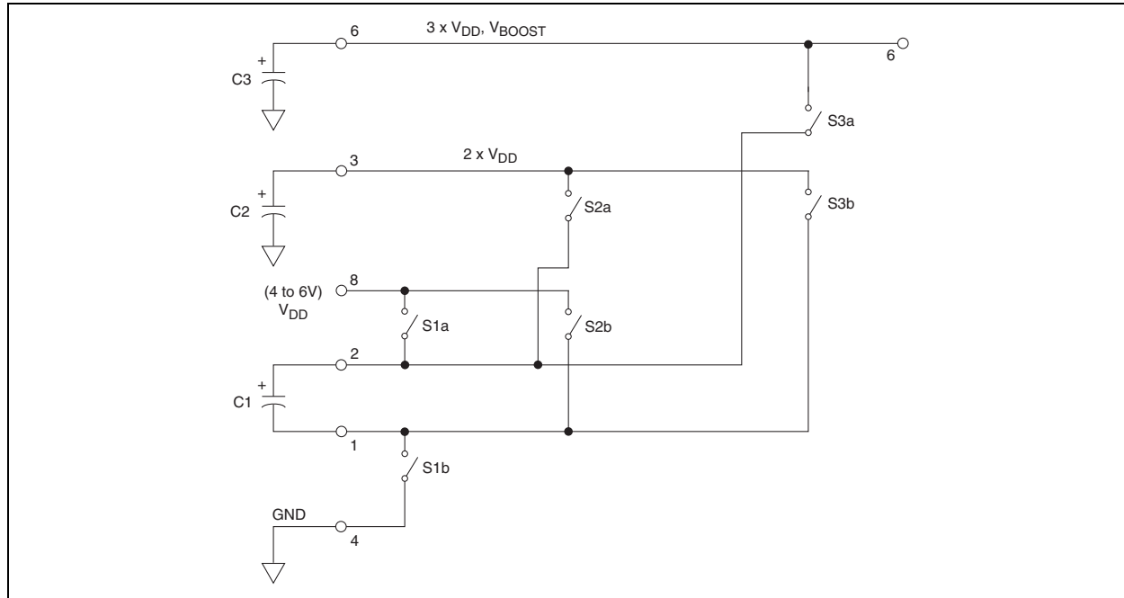
FIGURE 3-3: VOLTAGE BOOSTER
