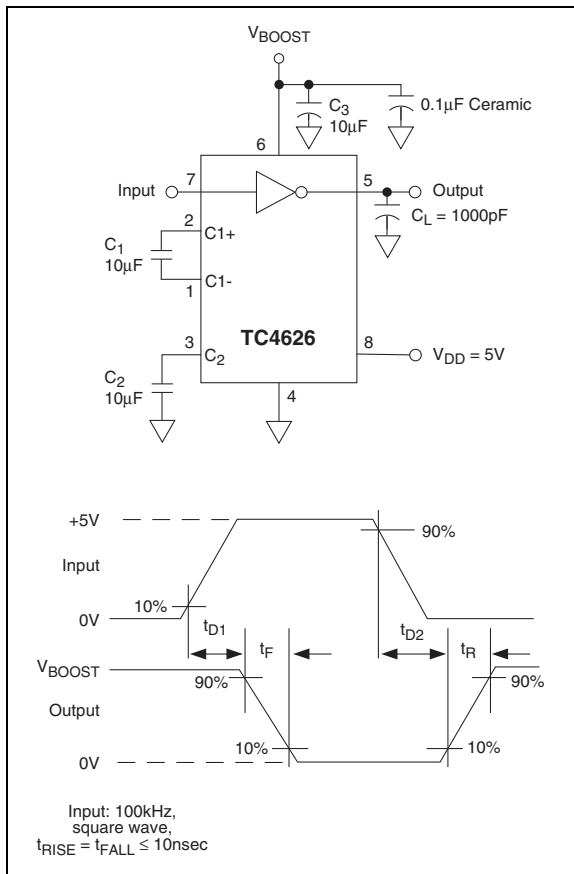
FIGURE 3-1: INVERTING DRIVER SWITCHING TIME
