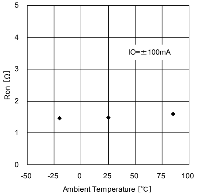
Figure 8. Output ON-Resistance Temperature Dependency (1ch-4ch driver block)
