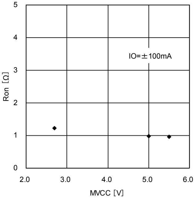
Figure 9. Output ON-Resistance MVCC Dependency (5ch,6ch driver block)
