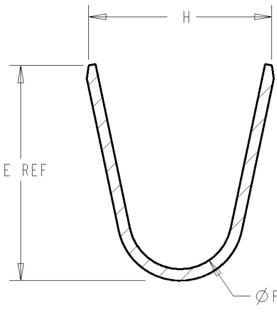
SECTION G-G
