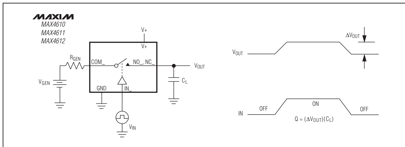
Figure 3. Charge Injection
