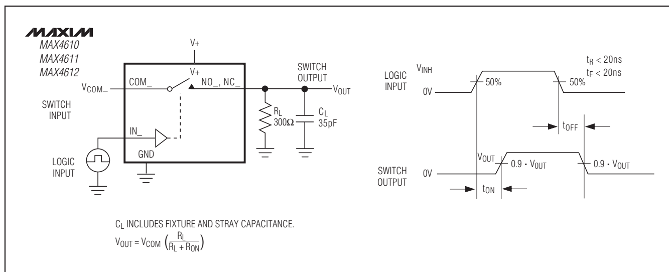
Figure 2. Switching Time
