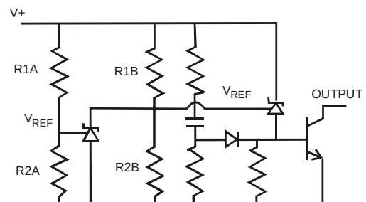
SERIES REGULATOR
