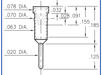
0400-0-15-XX-47-XX-04-0 Press-fit in .067 mounting hole.
