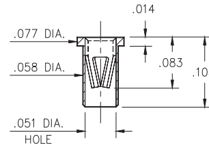
7305-0-15-XX-47-XX-10-0 Solder mount in .060 min. mounting hole Also available on 8mm wide carrier tape: 6,000 parts per 13" reel. Order as: 7305-0-57-XX-47-XX-10-0
