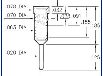
0400-0-15-XX-47-XX-04-0 Press-fit in .067 mounting hole.
