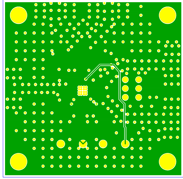
Figure 51. Evaluation Board Power Plane, Internal Layer 2
