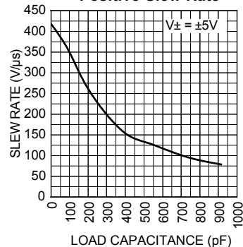
Positive Slew Rate
