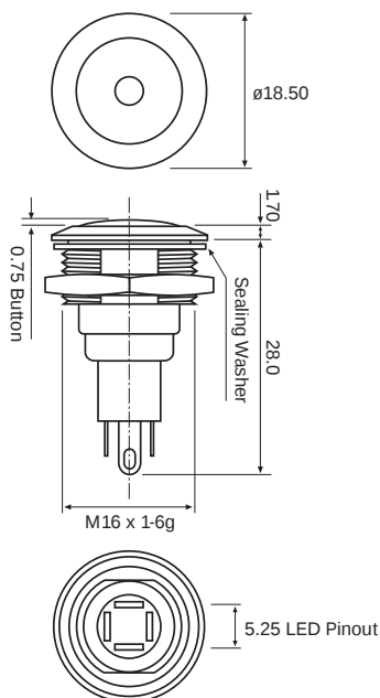
Illuminated Round Bezel
