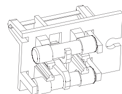
Metric dual fuse installation
