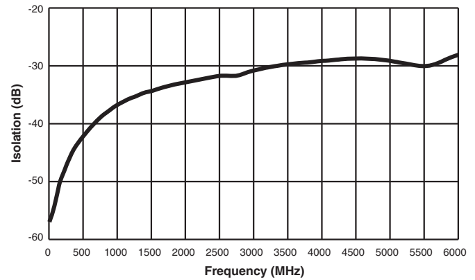
Isolation Pole to Pole (RF Note 5)
