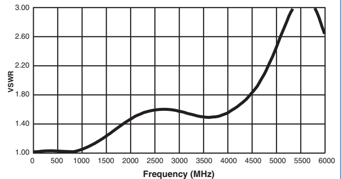
VSWR (RF Note 6)
