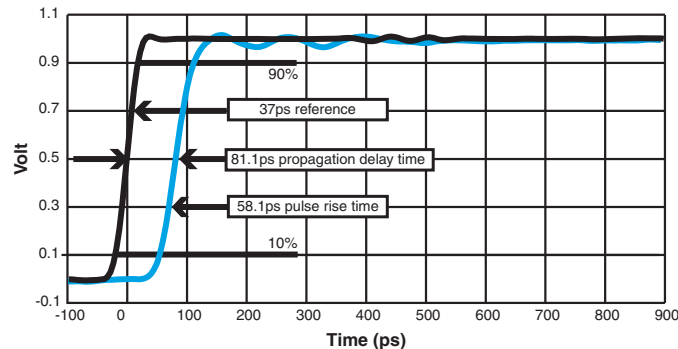
RF100 Time Response (RF Note 6)
