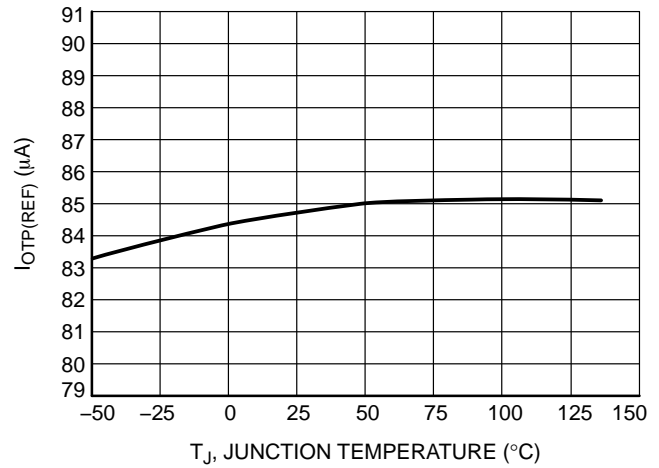
Figure 48. I OTP(REF) vs. Temperature
