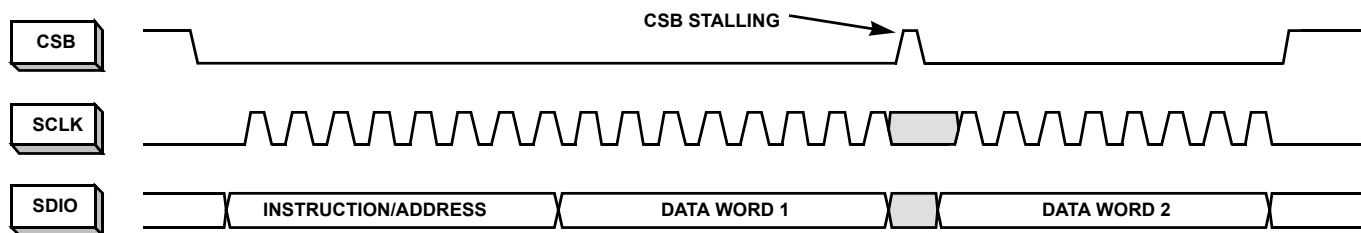
FIGURE 46. 2-BYTE TRANSFER
