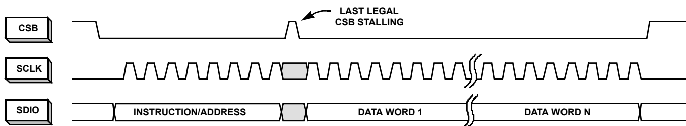
FIGURE 47. N-BYTE TRANSFER
