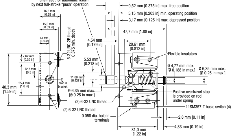
Figure 8. MICRO SWITCH™ 13AC1
