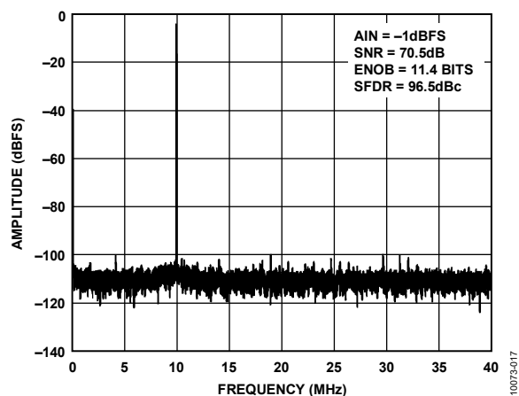
Figure 12. Single-Tone 16k FFT with f_{IN} = 70 \text{ MHz} , f_{SAMPLE} = 80 \text{ MSPS}
