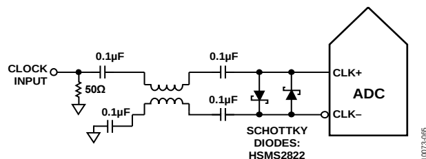
Figure 62. Balun-Coupled Differential Clock (Up to 1 GHz)
