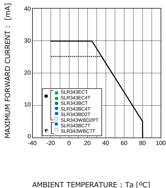
Fig.4 Derating
