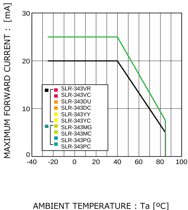
Fig.4 Derating
