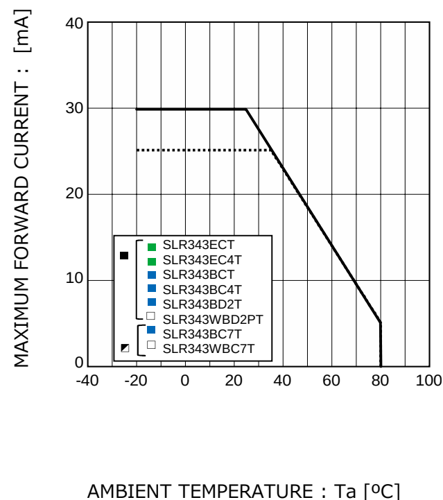
Fig.4 Derating
